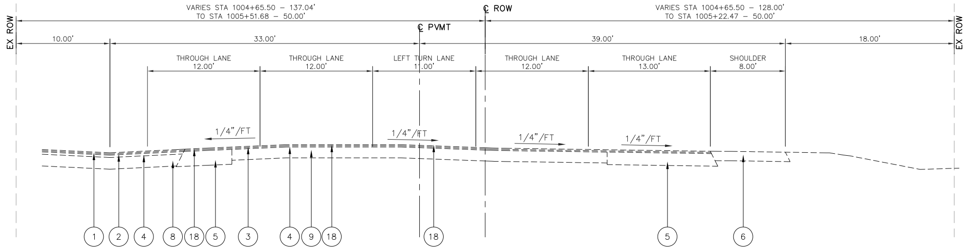
PR. TYPICAL SECTION - IL 3 (MISSISSIPPI AVE.) STA 1004+65.50 TO 1006+00 NOT TO SCALE
