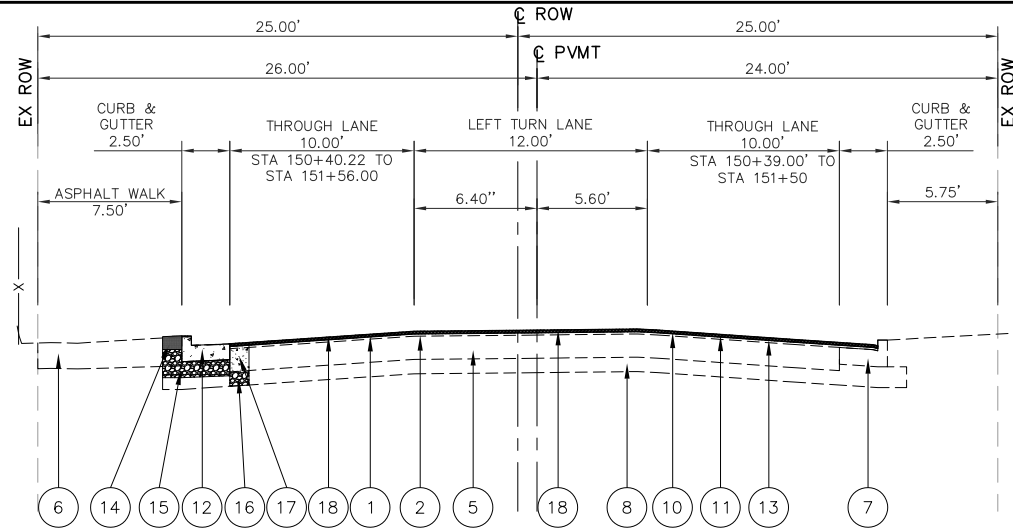
PR. TYPICAL SECTION - MONSANTO AVE. STA 150+39.00 TO 152+47.50 NOT TO SCALE
