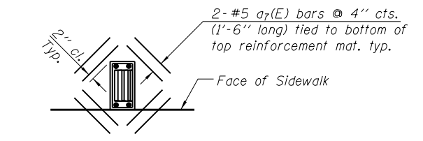
DETAIL AT SCUPPER
