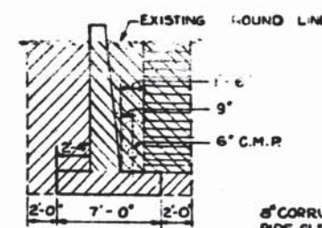
SECTION C-C TYPICAL RETAINING WALL SCALE: 3/16" = 1'-0"
