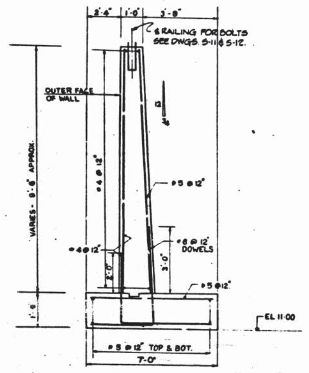
TYP SECTION THRU RETAINING WALL SCALE 1/2" = 1'-0"
