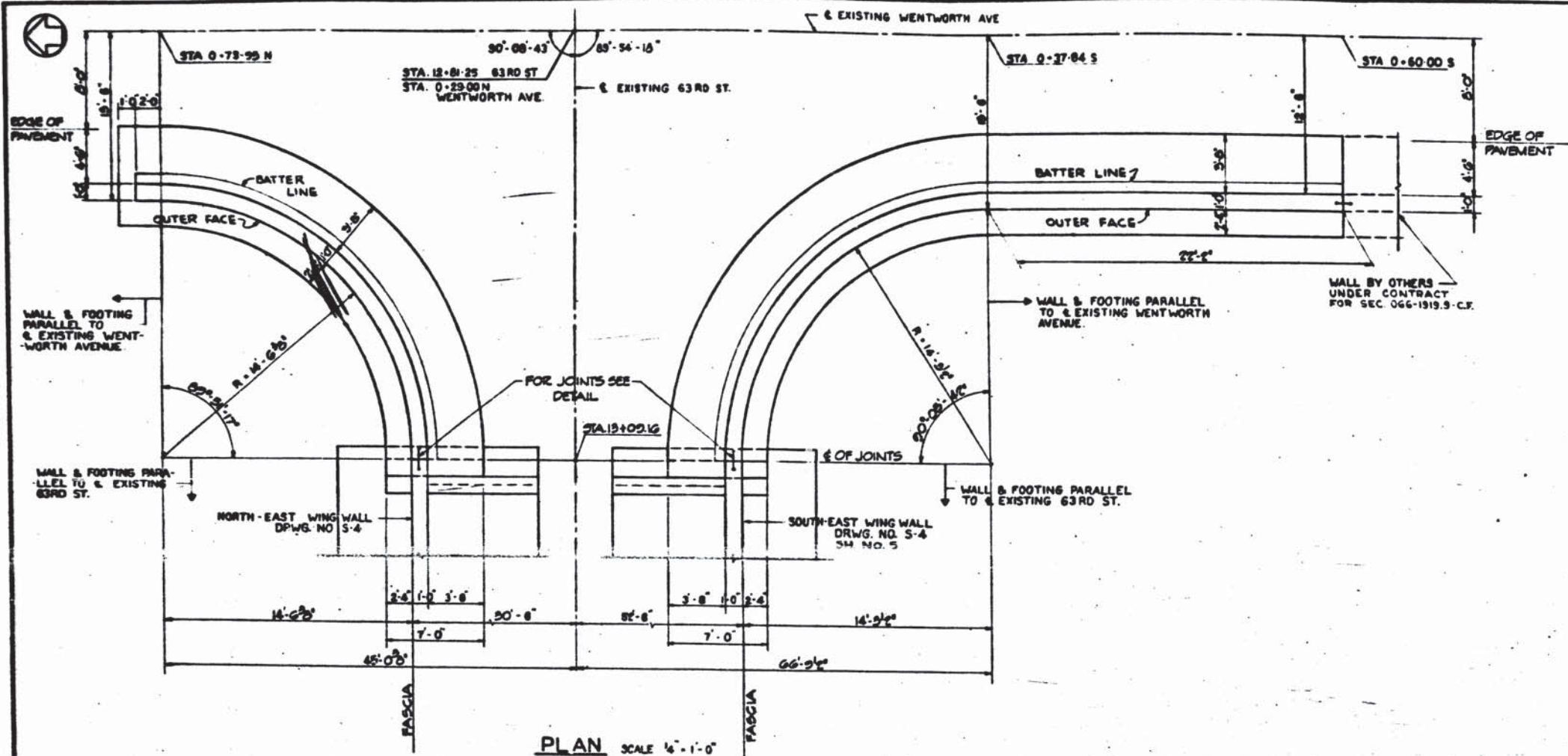
PLAN SCALE 1/4" = 1'-0"
