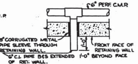
UNDERDRAIN OUTLET DETAIL SCALE: 1/2" = 1'-0"
