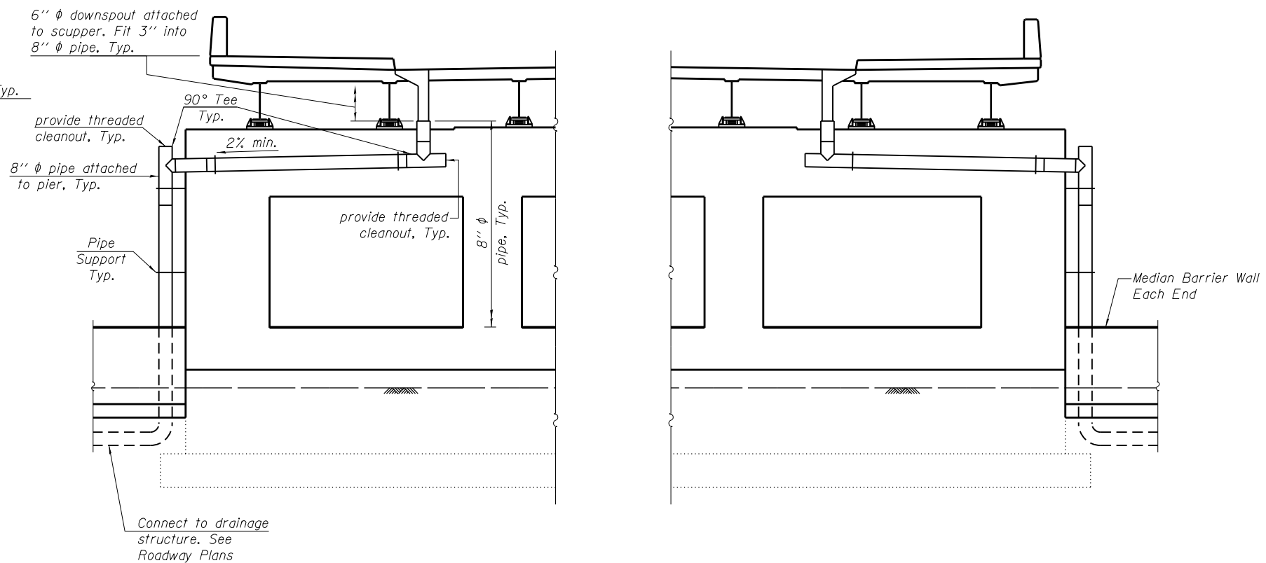
PARTIAL PIERS 1 & 4 ELEVATION
