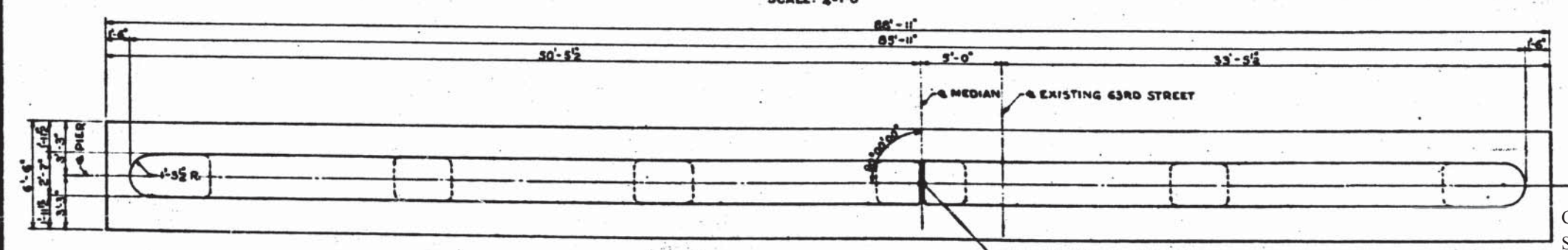
FOOTING PLAN SCALE: 1/8"=1'-0"
