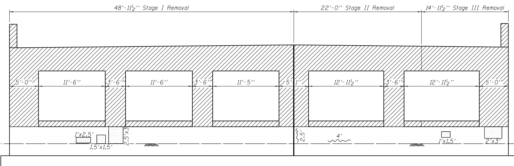
PIER 4 ELEVATION
