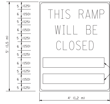
RAMP CLOSURE ADVANCE INFORMATION SIGN
