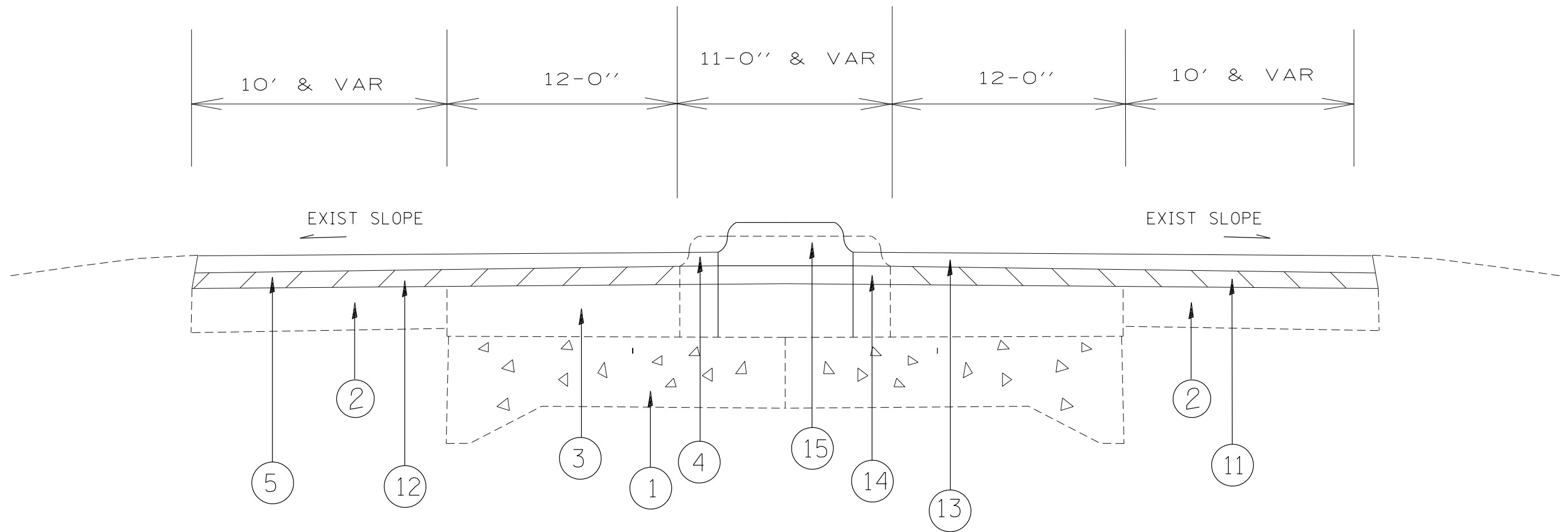
Typical section #1
