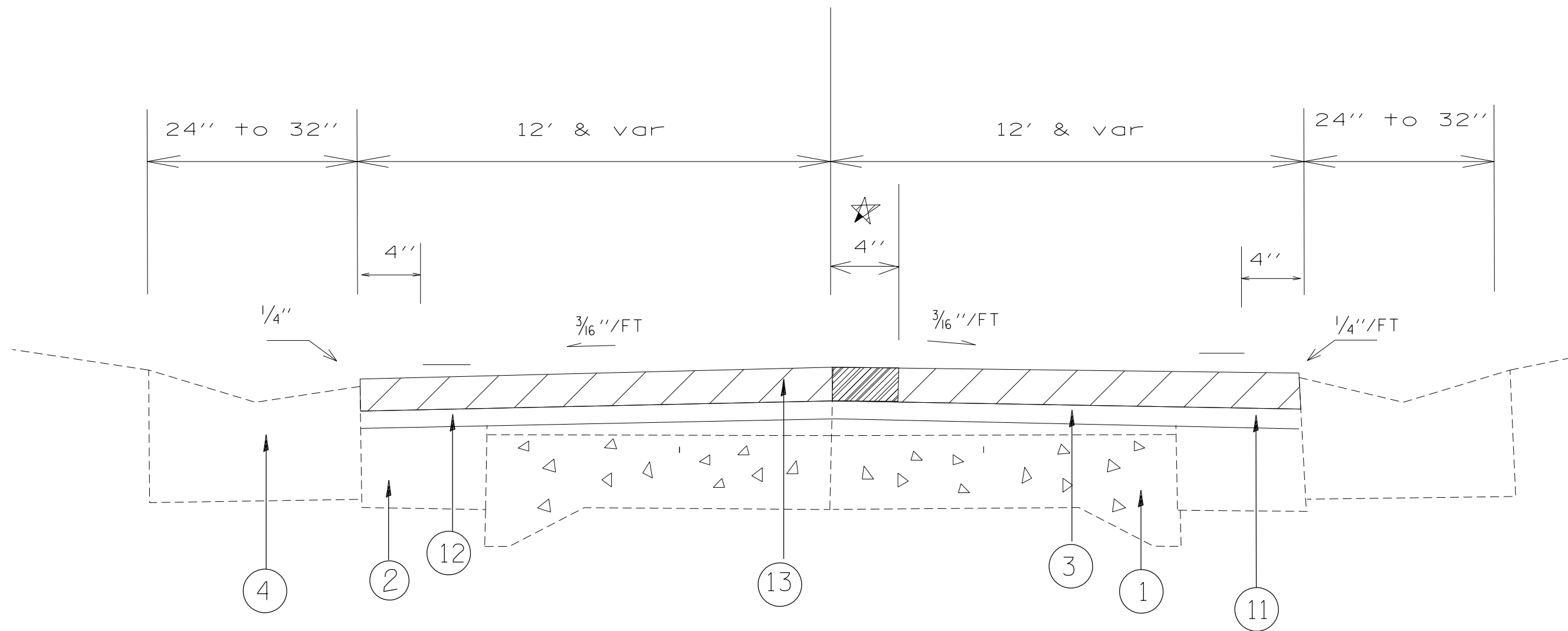
Typical section #3 US 150 LOOKING EAST
