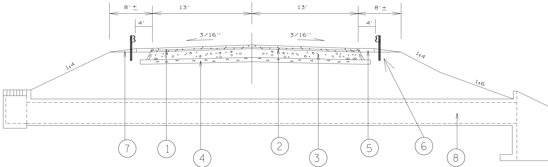
Typical section #5
