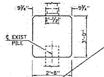
BRIDGE PIER MOUNT
