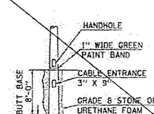
BUTT BASE
