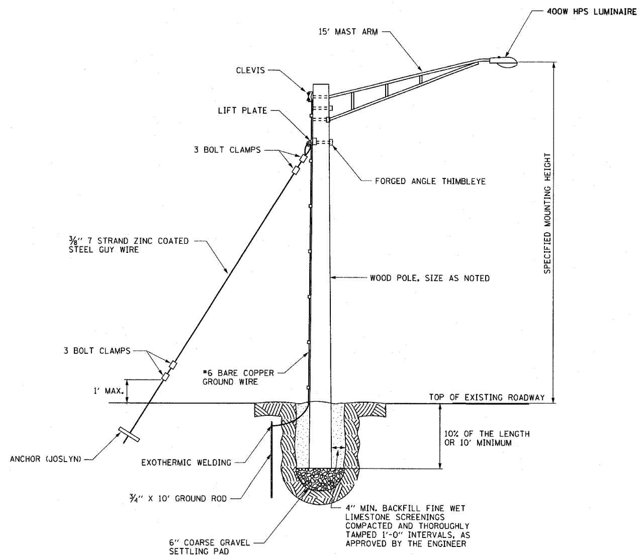
TEMPORARY LIGHT POLE DETAIL NOT TO SCALE
