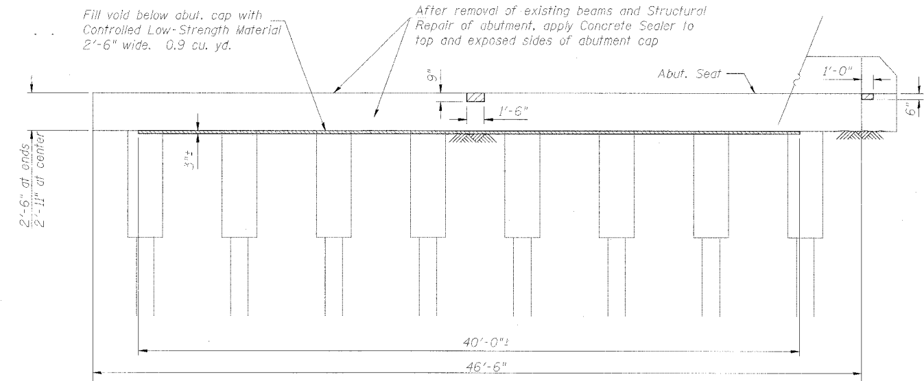
NORTH ABUTMENT
