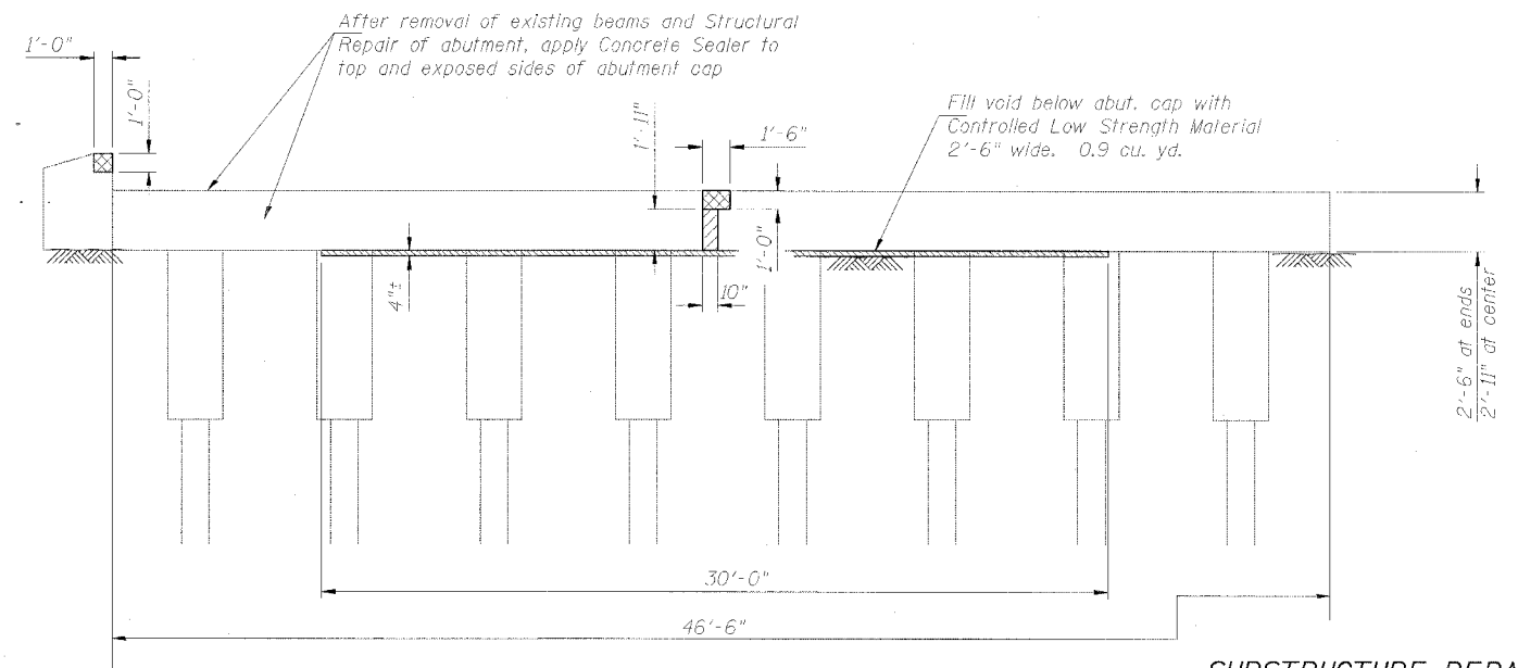
SOUTH ABUTMENT
