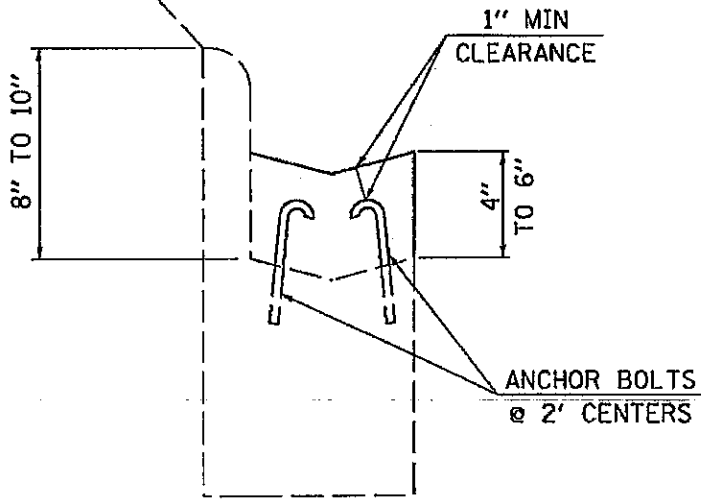
PROPOSED TYPE A GUTTER, SPECIAL
