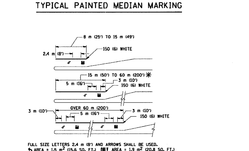
MEDIAN WITH TWO-WAY LEFT TURN LANE
