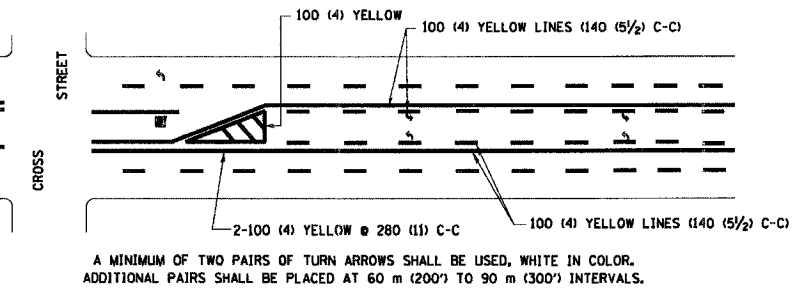
MEDIANS OVER 1.2 m (4') WIDE
