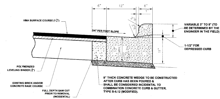
COMBINATION CONCRETE CURB & GUTTER TYPE B-6.12 (MODIFIED)
