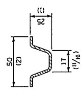
SECTION E-E Steel - 1.67 kg/m (1.12 lbs./ft.)
