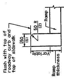
DETAIL OF SIDE CURB
