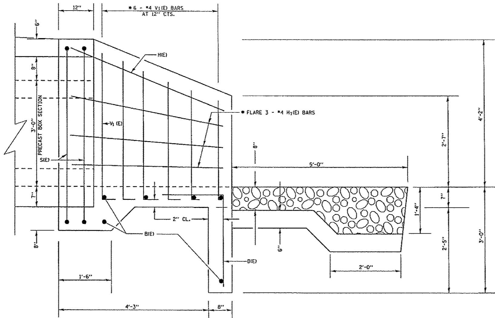
HALF SIDE ELEVATION
