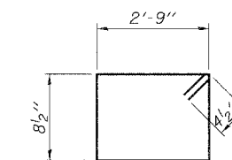
BARS s17(E)
