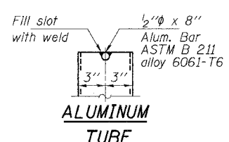
TOP PLAN
