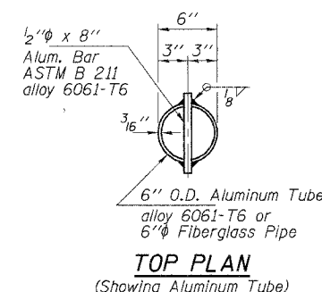
TOP PLAN
