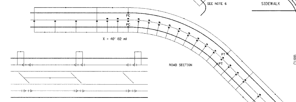
TYPICAL RAISED PAVEMENT MARKER INSTALLATION
