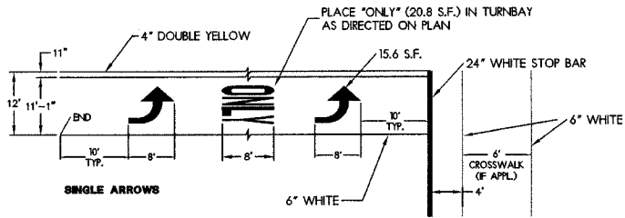
PAVEMENT MARKING DETAILS
