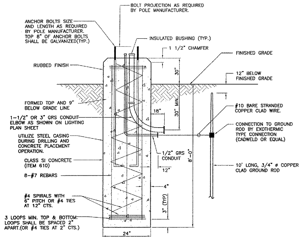
ELEVATIONS VIEW
