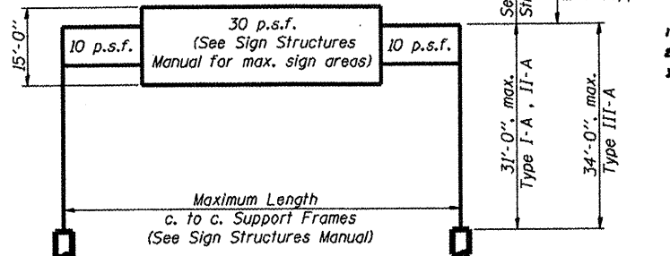
DESIGN WIND LOADING DIAGRAM
