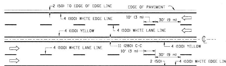
MULTI-LANE UNDIVIDED
