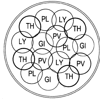
1 PLANTER BASKET PLANTING, TYP. OF 70 BASKETS (35 POLES) SCALE: N.T.S.
