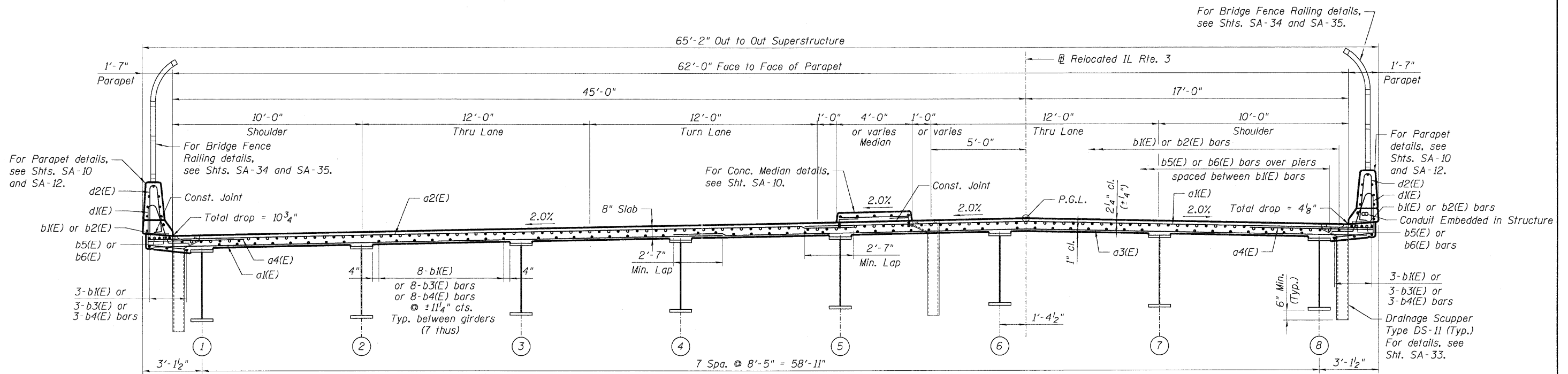
CROSS SECTION
