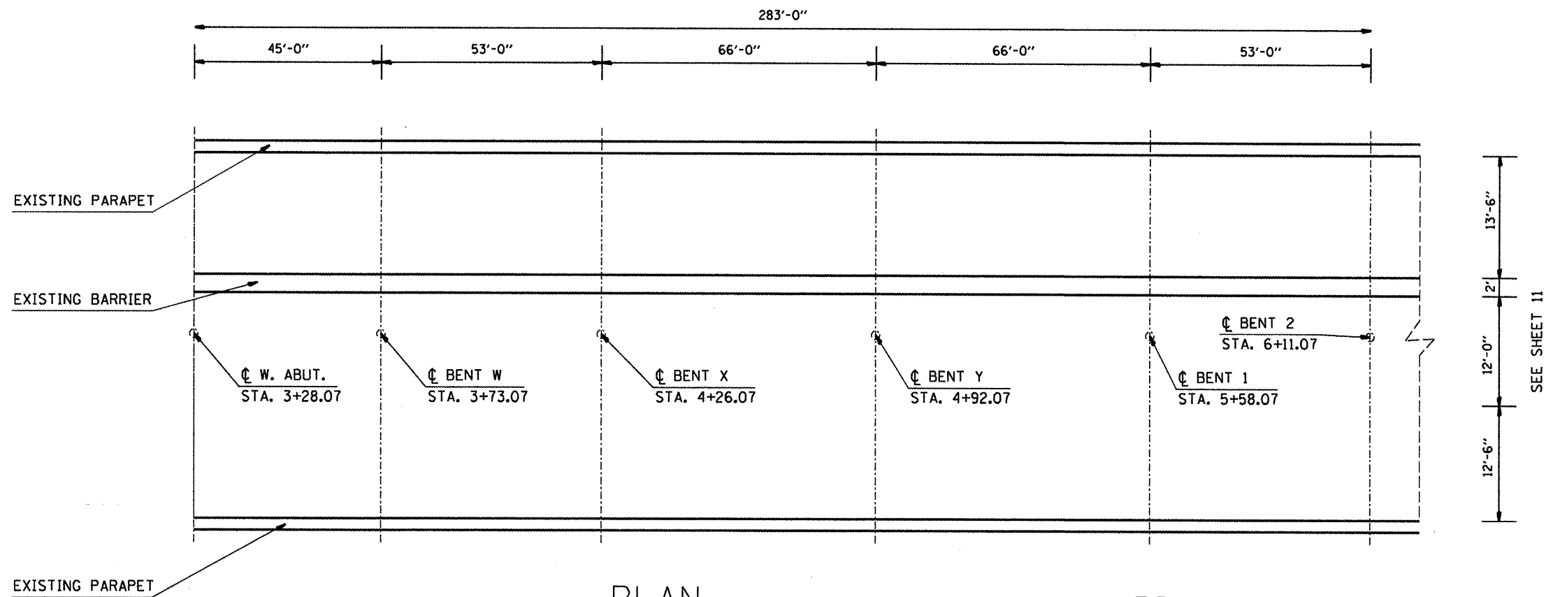
PLAN
