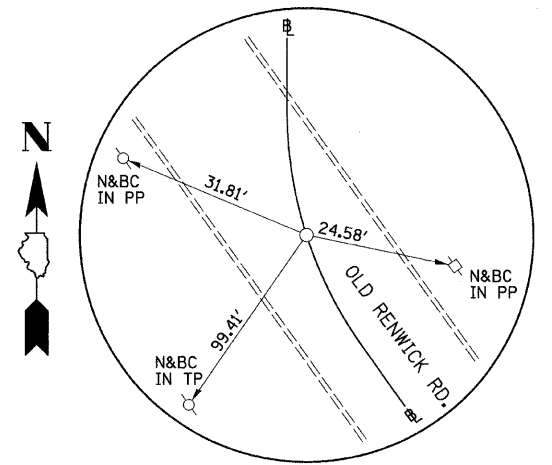
P.C. STA. 48+45.78 OLD RENWICK RD. N. 9840.348, E. 6180.470 (MAG NAIL)
