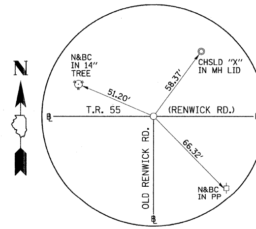
P.O.T. STA. 50+00.00 OLD RENWICK RD. N. 9982.784, E. 6136.743 (5/8" I-ROD)
