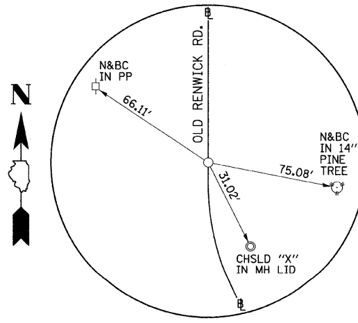
P.T. STA. 49+64.95 OLD RENWICK RD. N. 9947.733, E. 6136.455 (5/8" I-ROD)
