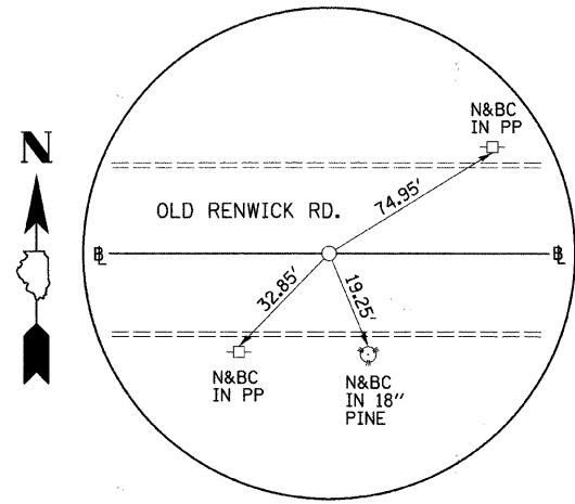
P.C. STA. 43+41.88 OLD RENWICK RD. N. 9547.533, E. 6581.711 (PK NAIL)
