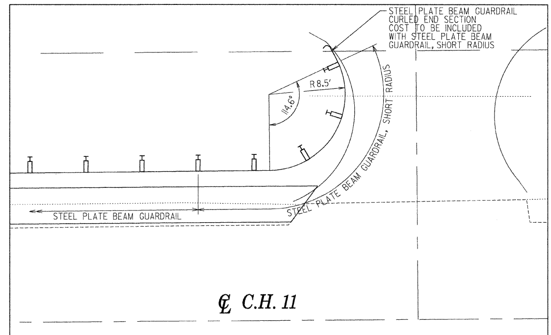
EAST GUARDRAIL DETAIL
