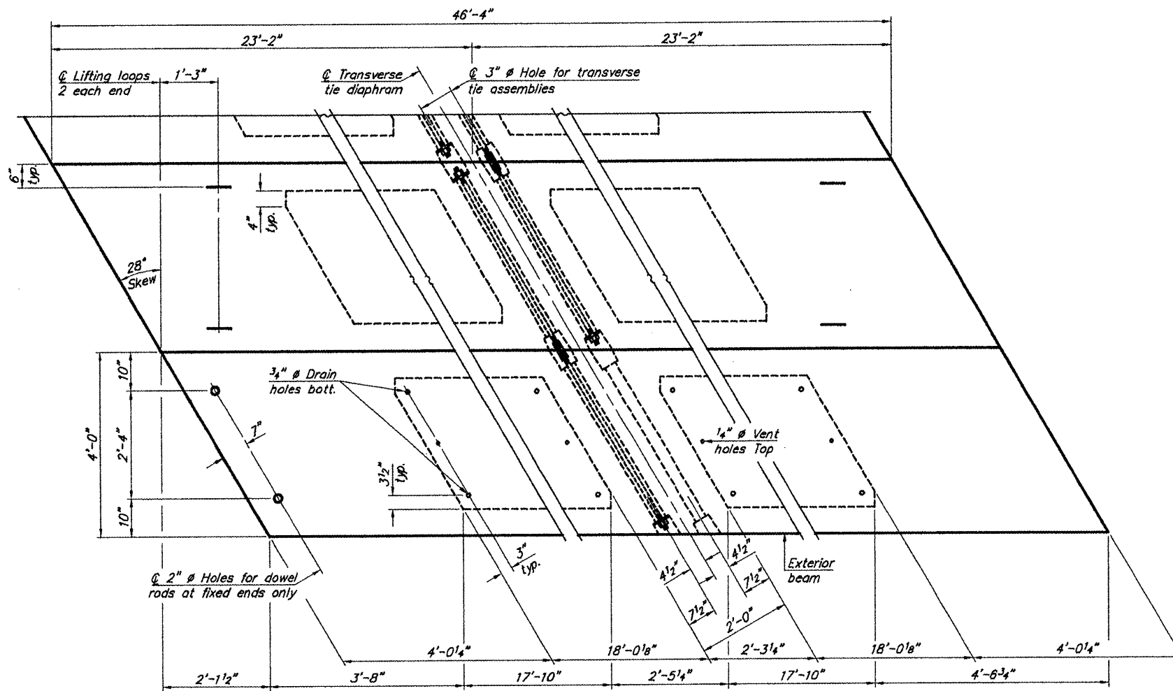
PLAN VIEW
