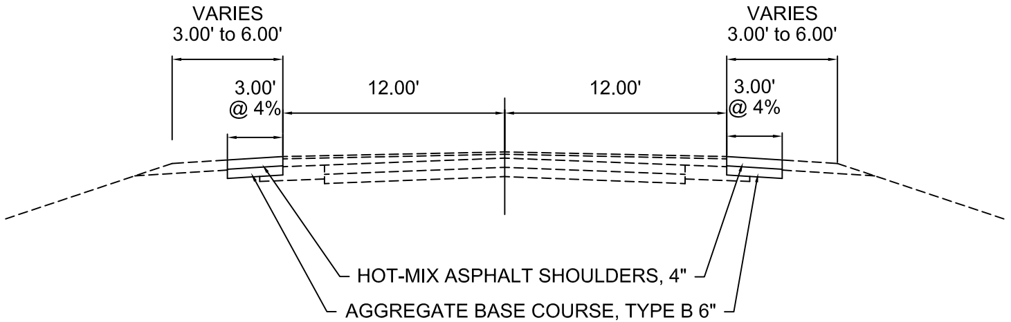
PROPOSED TYPICAL SECTION STA 106+84 TO STA 508+19
