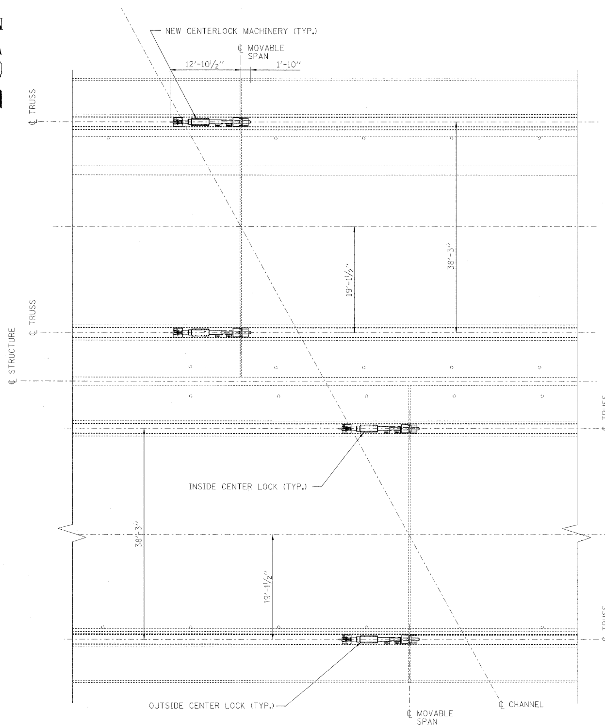
CENTER LOCK LOCATION PLAN
