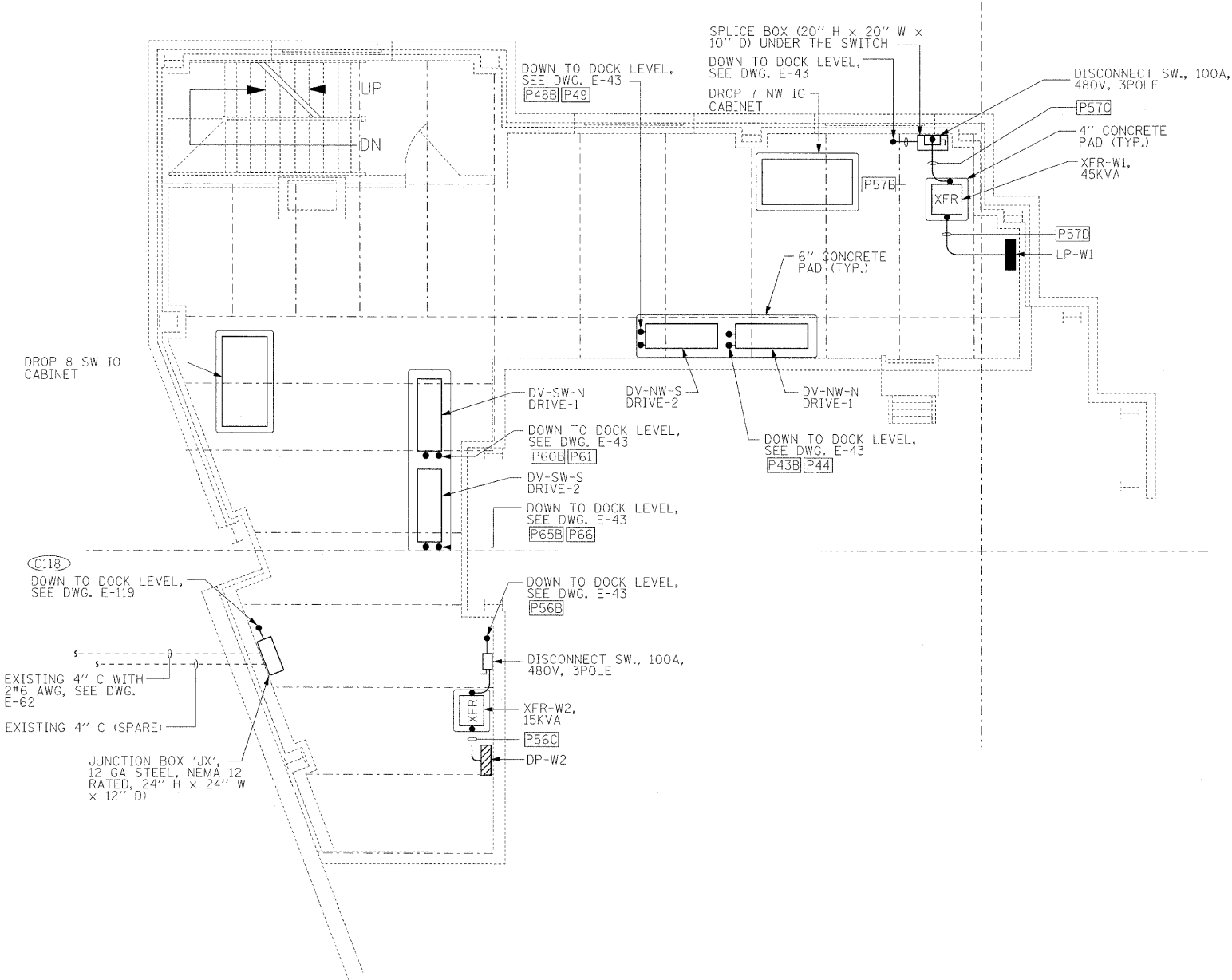
POWER PLAN 1/4"=1'-0"
