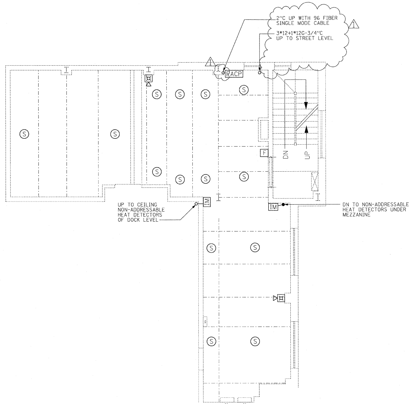
AUXILIARY SYSTEMS PLAN 1/4" = 1'-0"
