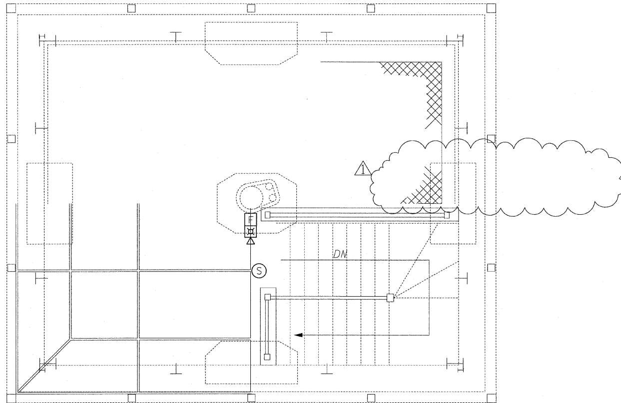
AUXILIARY SYSTEMS PLAN 1/2" = 1'-0"
