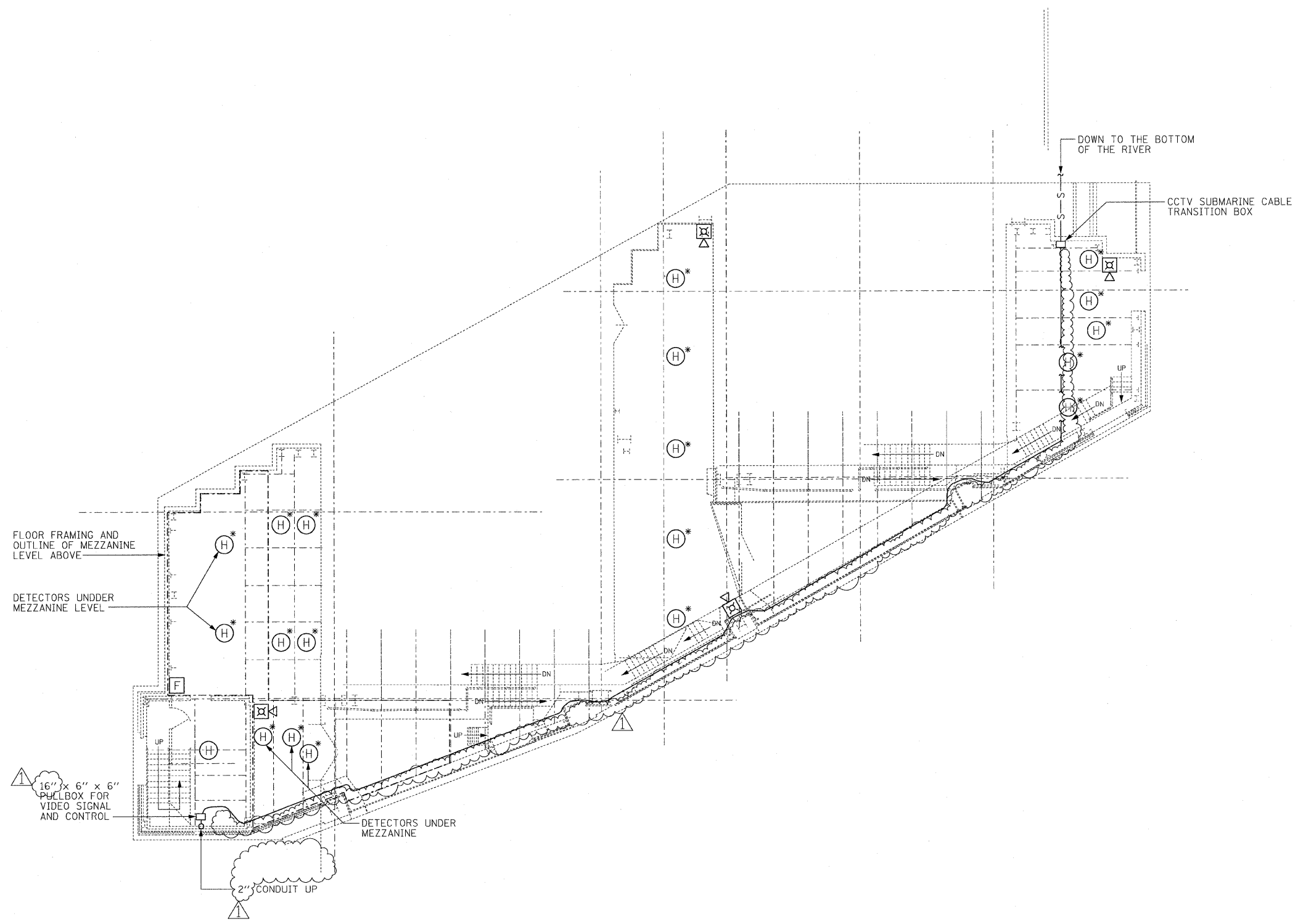
AUXILIARY SYSTEMS PLAN 1/8" = 1'-0"
