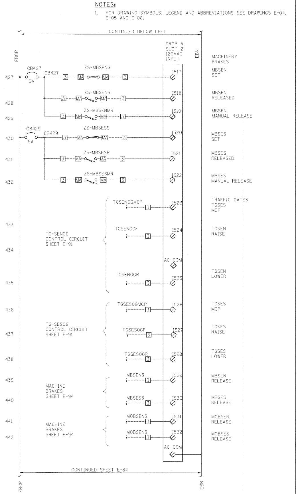
DROP 5 SOUTHEAST PLC I/O CABINET
