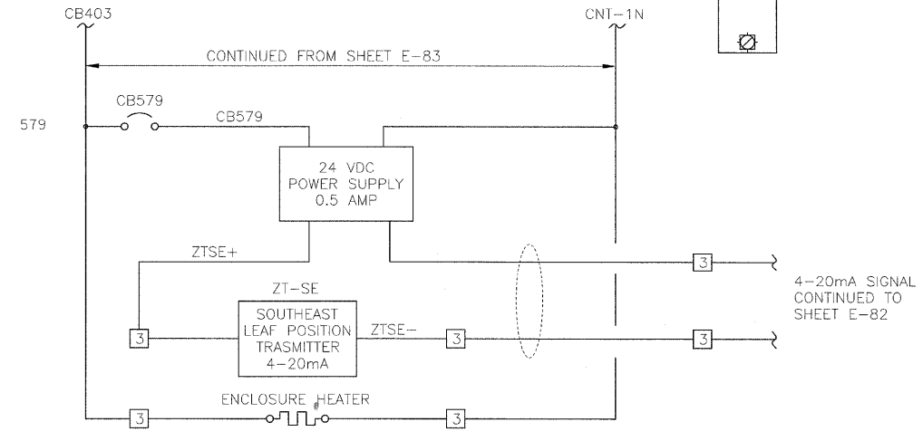
SOUTHEAST LEAF POSITION TRANSMITTER
