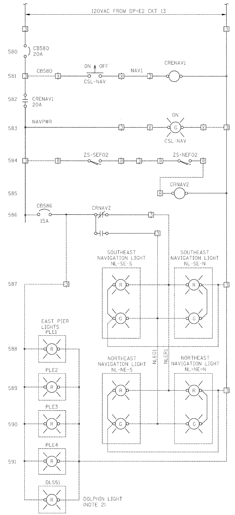
DROP 5 SOUTHEAST PLC I/O CABINET
