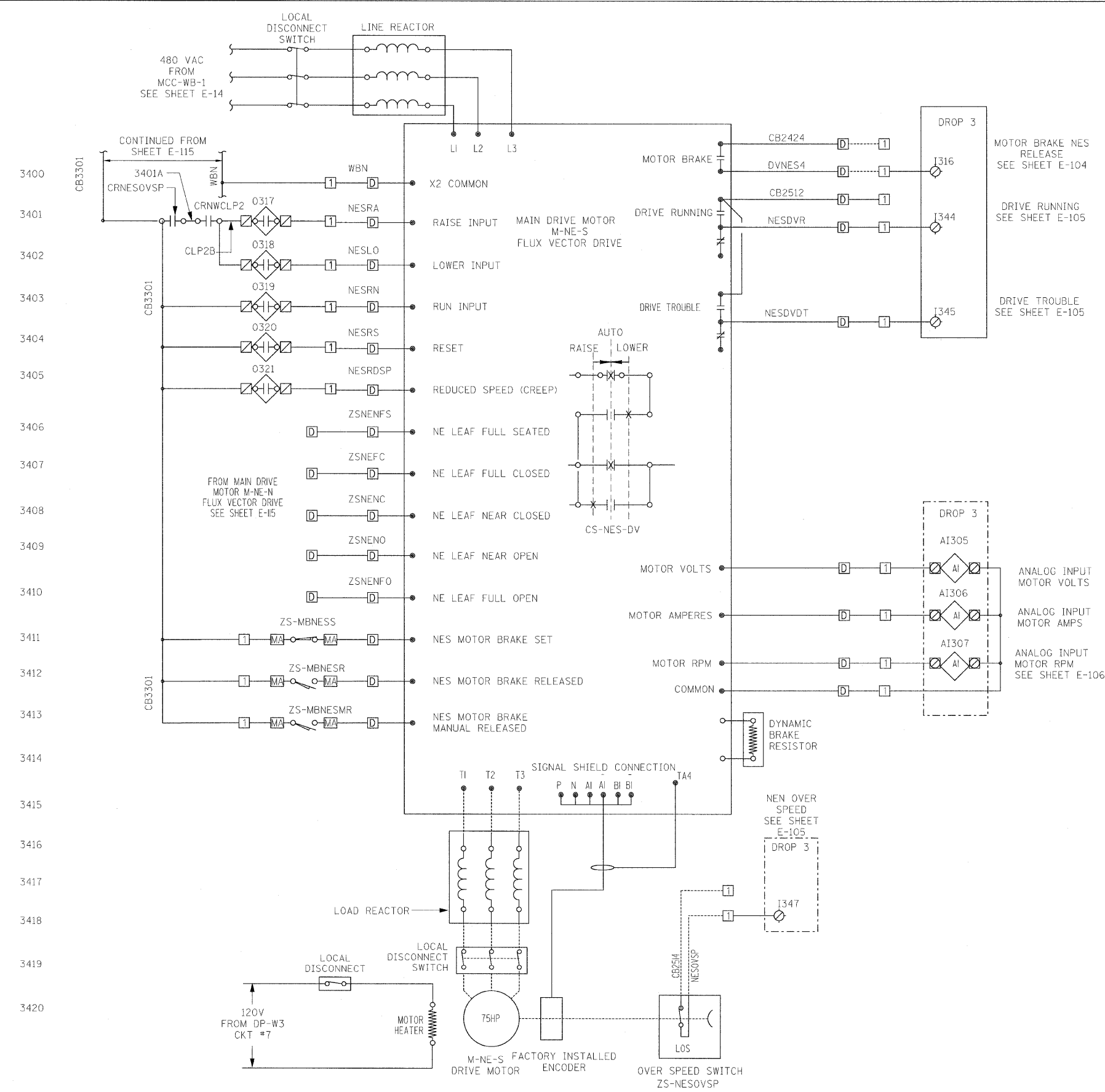
WESTBOUND MAIN MOTOR NES DRIVE
