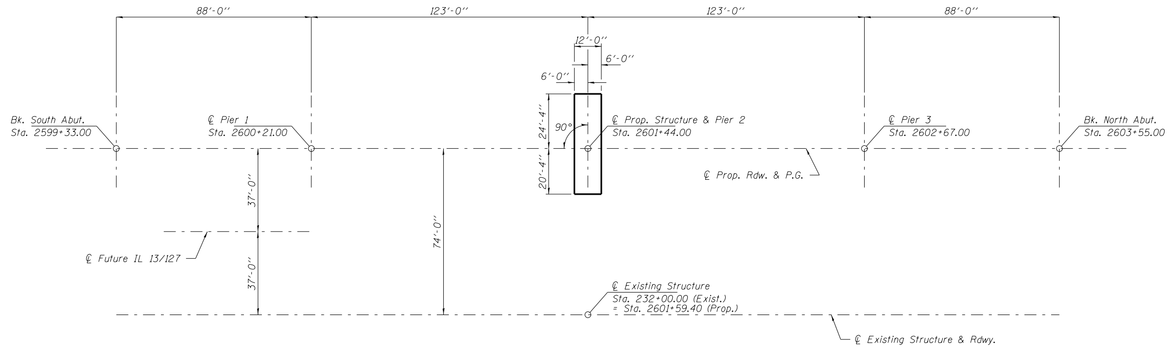
FOOTING LAYOUT
