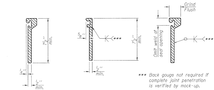
ROLLLED EXTRUDED RAIL
