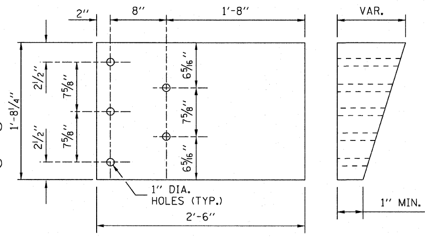
PARAPET WOOD BLOCK-OUT DETAIL
