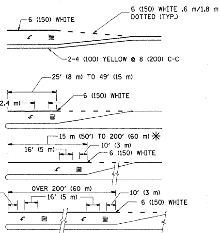
TYPICAL PAINTED MEDIAN MARKING
