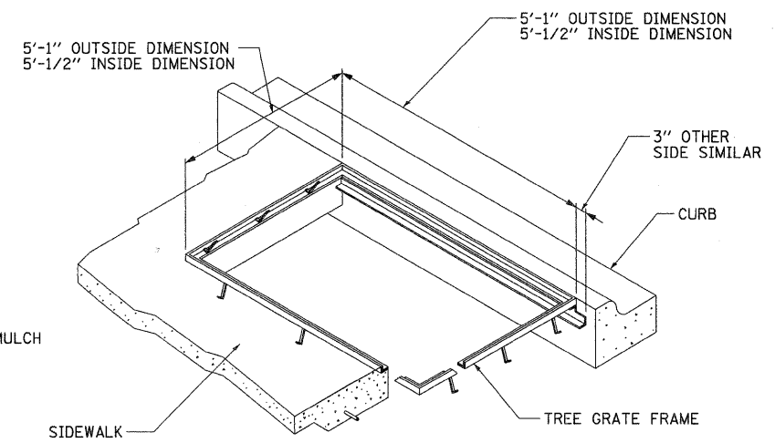
TREE GRATE FRAM INSTALLATION AT CURB N.T.S.
