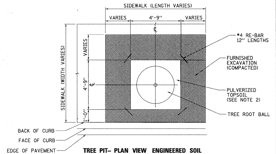
TREE PIT- PLAN VIEW ENGINEERED SOIL N.T.S.
