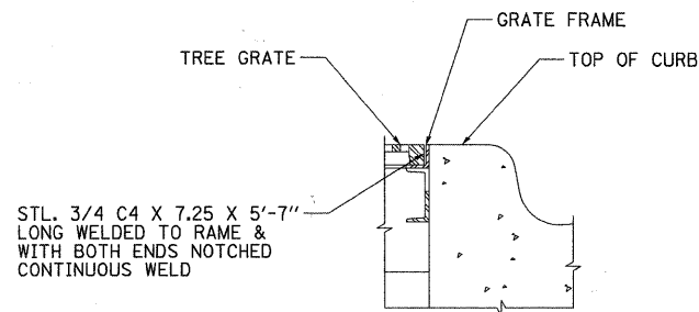
DETAIL 2: GRATE FRAME ABUTTING BACK OF CONCRETE CURB N.T.S.
