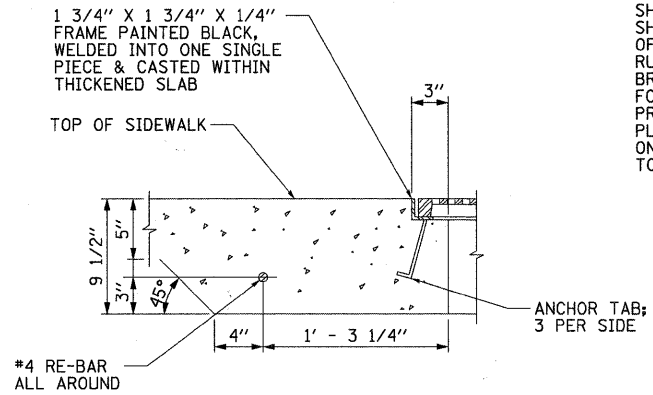
DETAIL 1: GRATE FRAME AT THICKENED SLAB N.T.S.
