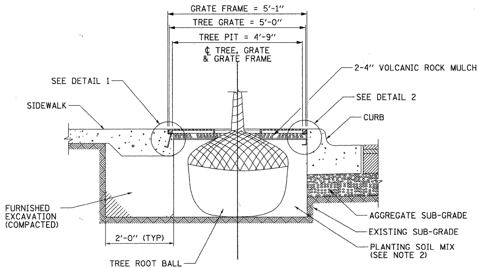
TREE PIT - CROSS SECTION (WITH STEEL TREE GRATE FRAME) N.T.S.
