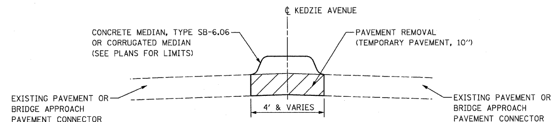
KEDZIE AVENUE MEDIAN RESTORATION TYPICAL SECTION STA. 13+10 TO STA. 15+85.83 STA. 19+92.18 TO STA. 22+70
