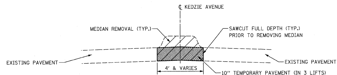
KEDZIE AVENUE TEMPORARY PAVEMENT TYPICAL SECTION STA. 13+10 TO STA. 15+75.83 STA. 20+02.18 TO STA. 22+70
