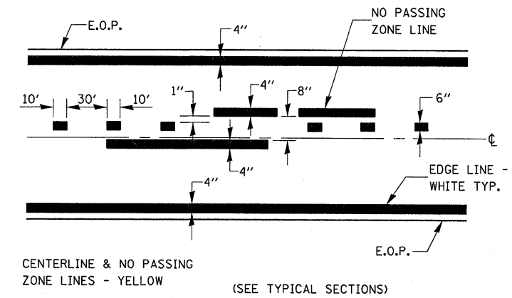
PAVEMENT MARKING
