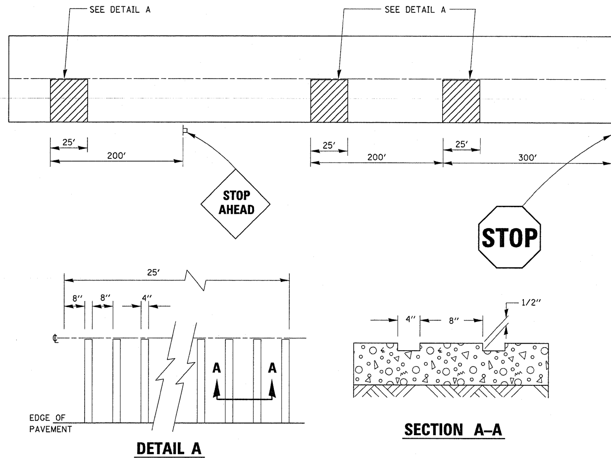
TYPICAL GROOVED RUMBLE STRIP APPLICATION IN ADVANCE OF AN INTERSECTION
