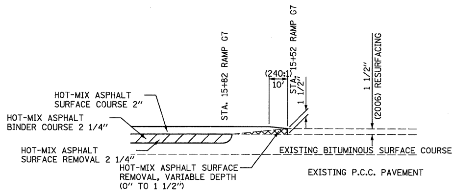
JOINT DETAIL ⑩
