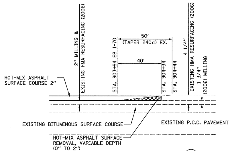
JOINT DETAIL ⑪
