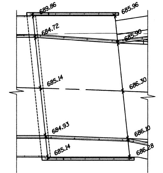
EAST APPROACH PAVEMENT PLAN
