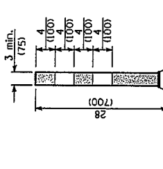
FLEXIBLE DELINEATOR
