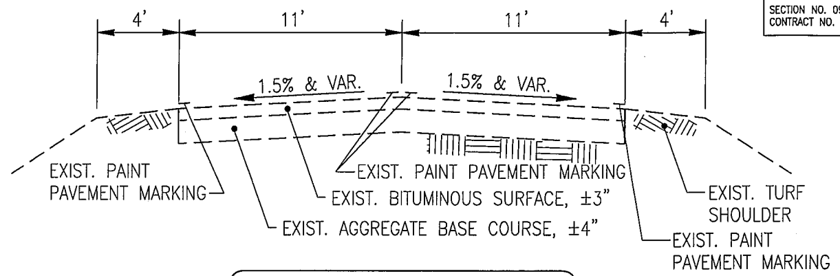
EXISTING TYPICAL SECTION FRONTAGE ROAD STA 0+00 TO 23+40
