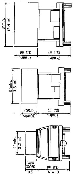
TYPE C TRAILER MOUNTED
