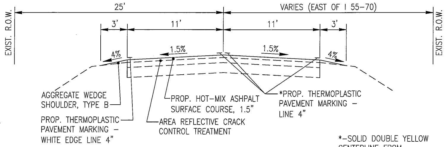
PROPOSED TYPICAL SECTION FRONTAGE ROAD STA 0+30 TO 23+10
