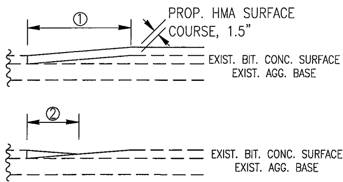
PROPOSED BUTT JOINT
