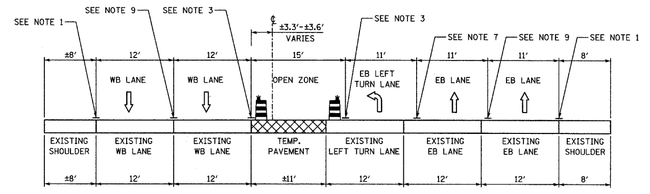
D-D PRE STAGE B: W. 75TH STREET; STA. 146+10 TO STA. 147+50
