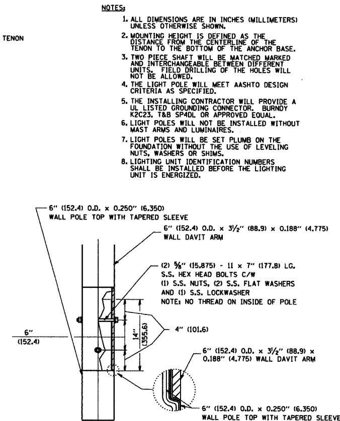
DAVIT ARM CONNECTION [14" (355.6) OVERLAP SHOWN]
