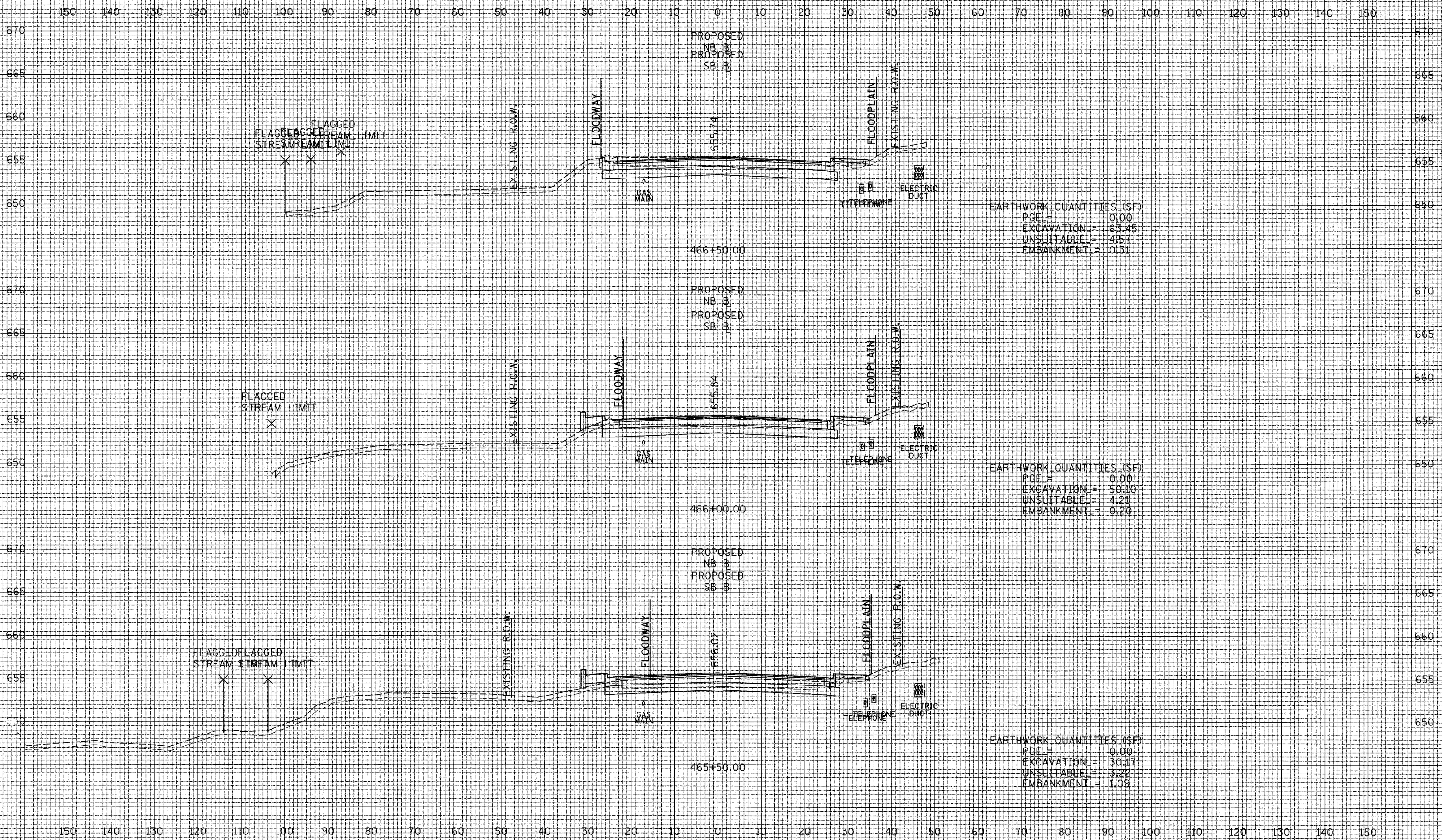
WASHINGTON ST. CROSS SECTION
