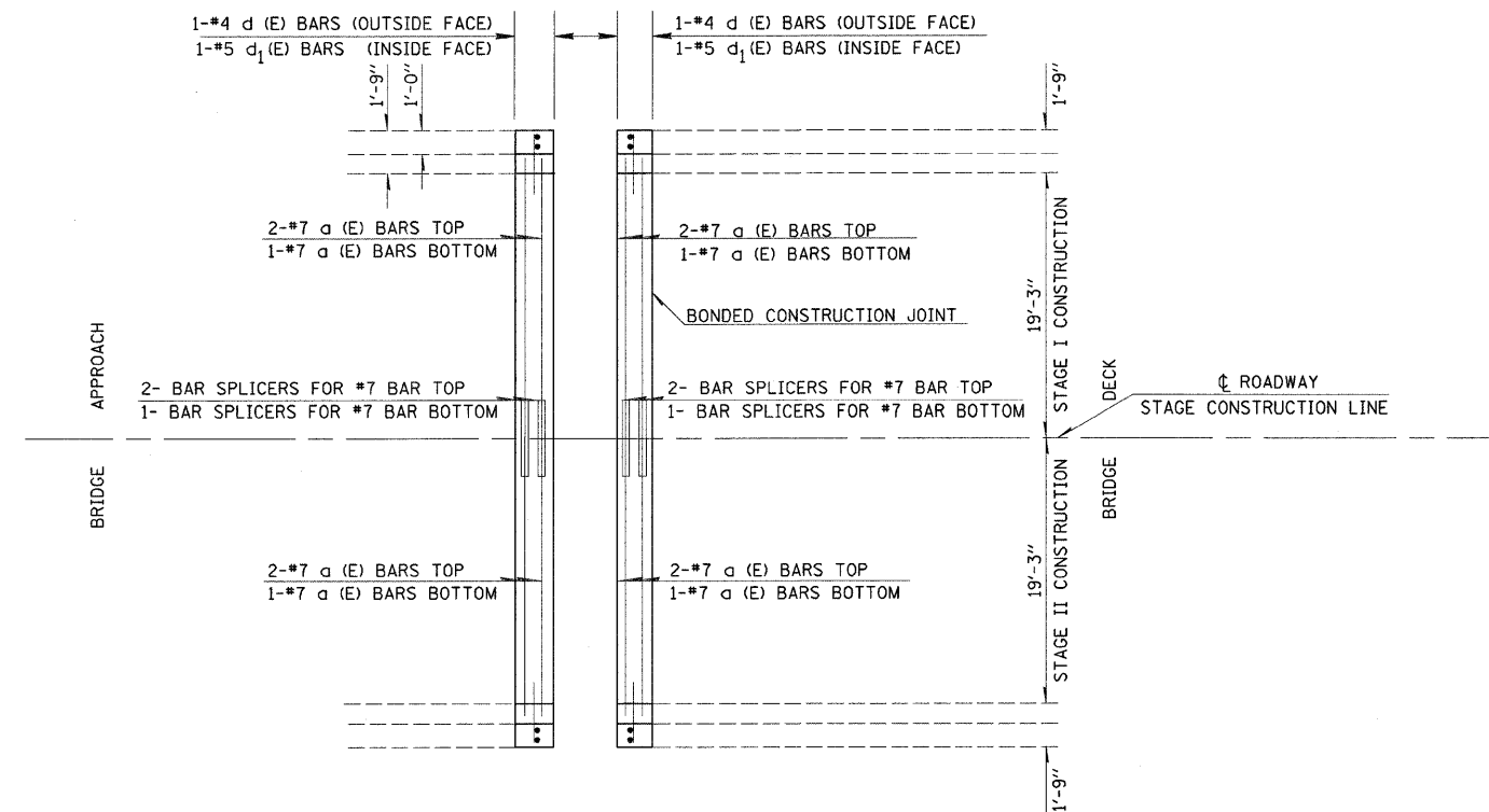
REINFORCEMENT DETAIL BENT 4 (BENT 9 SIMILAR)
