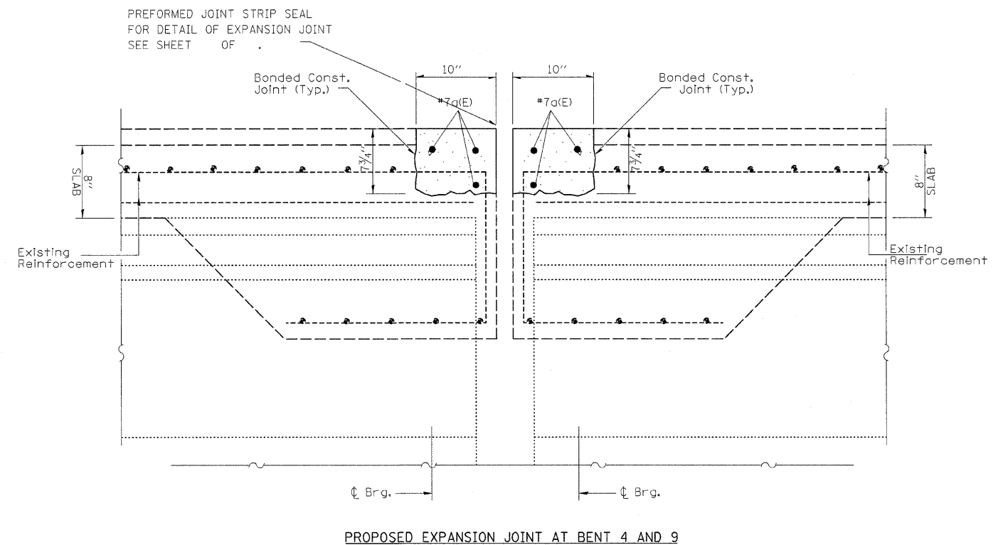
REINFORCEMENT DETAIL BENT 4 (BENT 9 SIMILAR)
